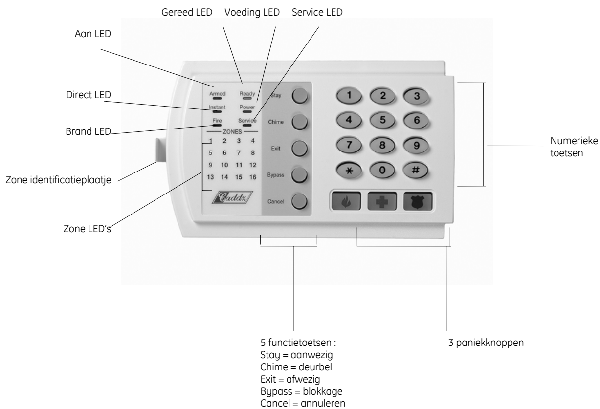
NX-116 LED codeklavier
